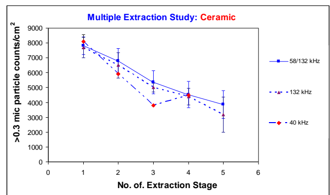
Fig.1 Multiple-extraction comparison of various ultrasonic frequencies with respect to particle removal efficiency and erosion propensity for ceramic components
