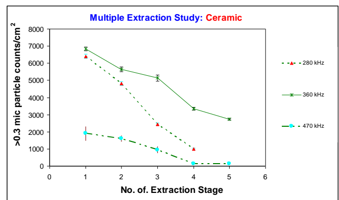
Fig.2 Multiple-extraction comparison of various megasonic frequencies with respect to particle removal efficiency and erosion propensity for ceramic components
