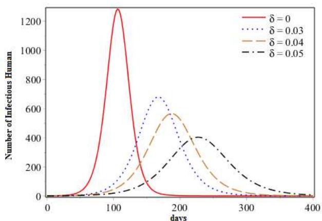
Figure 4. The intensity of infection is reduced when a constant parameter is given.
