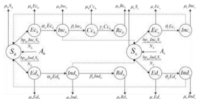
Figure 1. Transition diagram of the model. The solid lines indicate the change in state. The dashed lines indicate interaction between populations.
