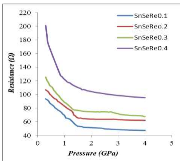
Figure 3. Variation of electrical resistance with pressure for SnSeRe( x=0.1, 0.2, 0.3, 0.4 ) single crystals using Bridgman anvils
