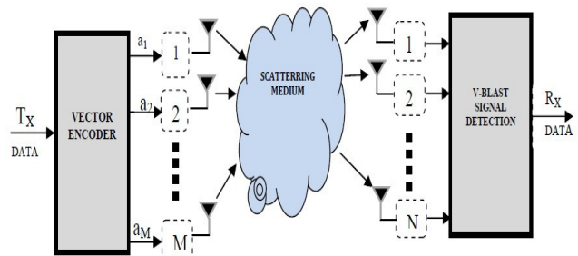
Figure 1. The V-BLAST MIMO Channel Model.
