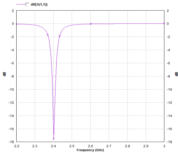
Figure 5. Return loss curve for Strip Feed.
