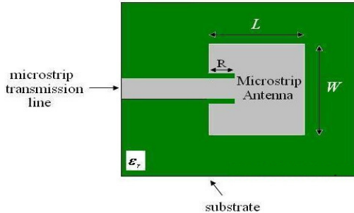
Figure 3. Rectangular Patch Antenna with Inset Line Feed.
