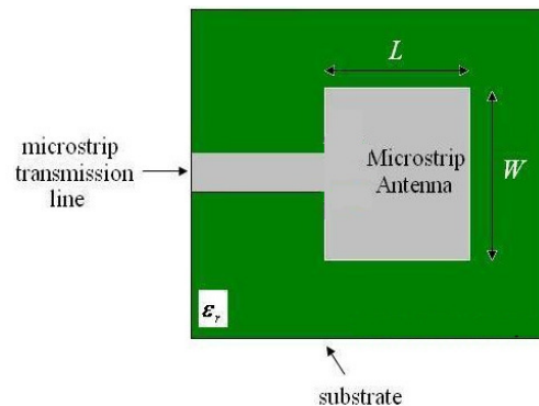
Figure 2. Rectangular Patch Antenna with Strip Feed.
