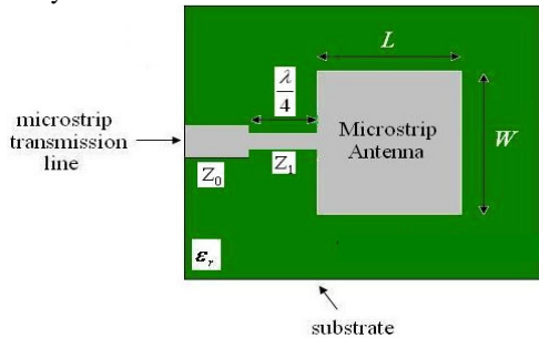
Figure 4. Rectangular Patch Antenna with Quarterwave Line Feed.
