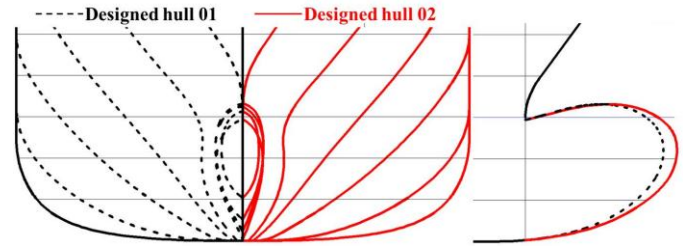
Figure 3. Ship lines of the designed hull 01 and 02
