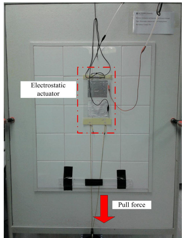
Fig. 2. Experiment setup photograph showing electrostatic actuator B7x4 on ceramic tiles wall surface.
