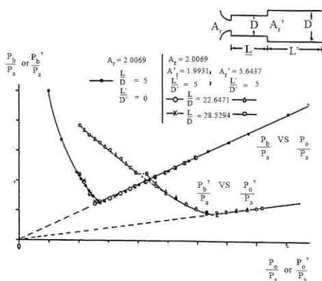
Figure 7. Base pressure at valve pipe-vent pipe junction.
