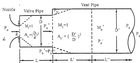
Figure 9. The schematic diagram of the vent pipe.
