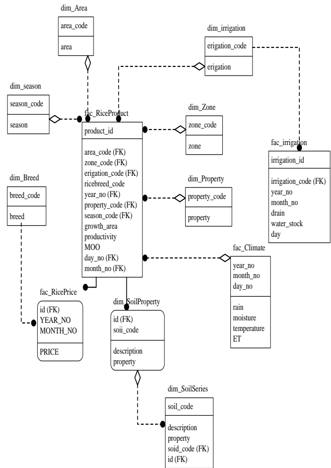
Figure 2: DWR Snowflake Schema
