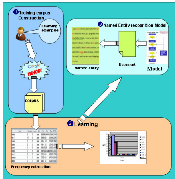
FIG 1 NER FLOW DIAGRAM
