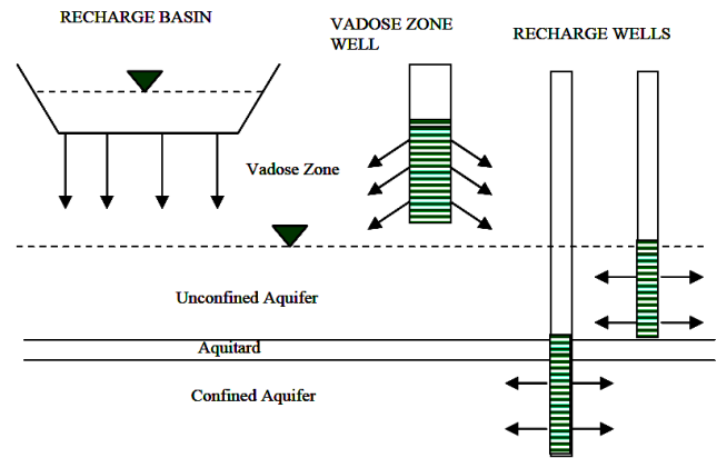
Figure 2. Major methods for aquifer recharge..
