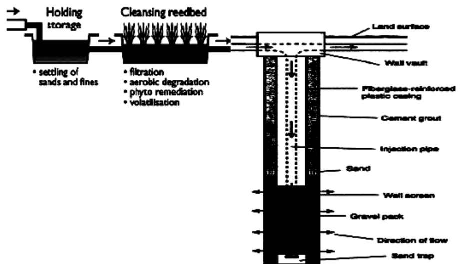
Figure 3. Constructed wetland with perforated drain in gravel layer on bottom discharged in vadose zone well for aquifer recharge.
