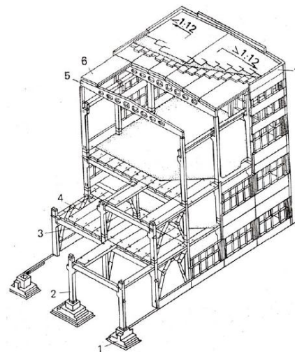
Figure 2. Multistory concrete prefabricated industrial building: 1- foundation, 2 - column, 3- beam, 4 - strengthen ties, 5 - beam, 6 - roof panel
