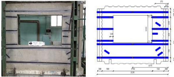
Figure 8. Experimental stand [3]
