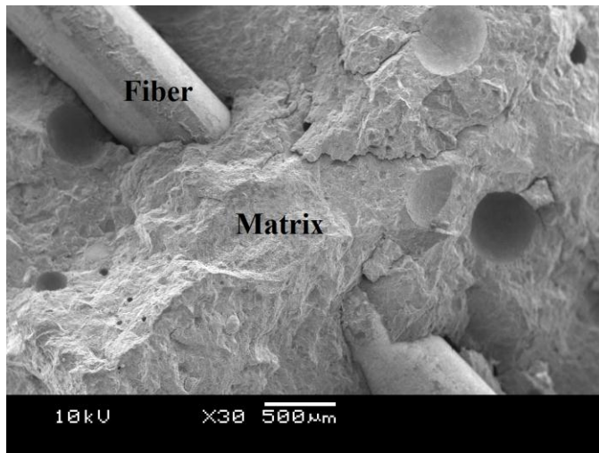
Figure 1. SEM image of steel fiber embedded in mortar
