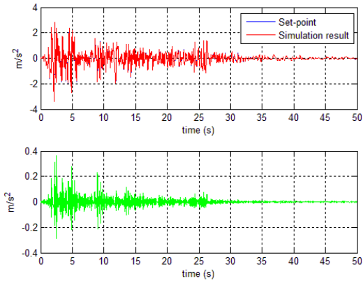
Figure 14. Acceleration (sample seismic event)
