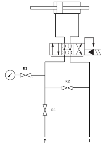
Figure 9. Hydraulic scheme
