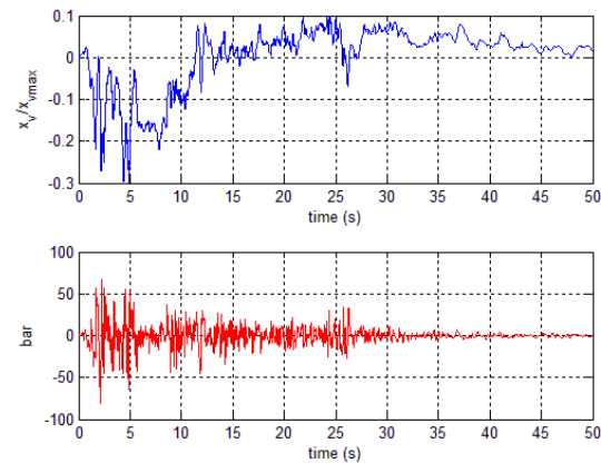
Figure 15. Valve opening ratio ( X_v/X_{v \max} ), pressure drop.
