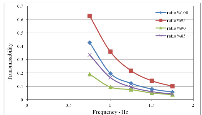
Fig. 2: Transmissibility against frequency for different ratio of foam in FFFluid pad sample.
