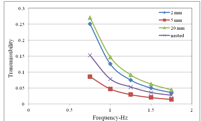
Fig. 1: Transmissibility against frequency for different size of foam in FFFluid pad sample.
