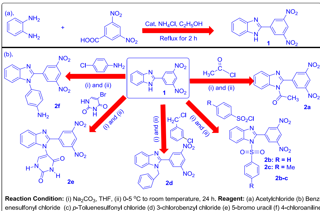
Scheme 1: (a). Synthetic pathway to Precursor 1 (b). Synthesis of the Final Benimidazole Products 2a-f
