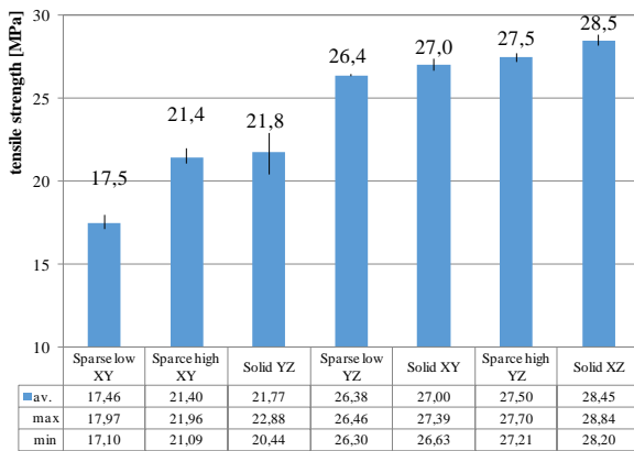
Figure 10. Average tensile strength in increasing order.
