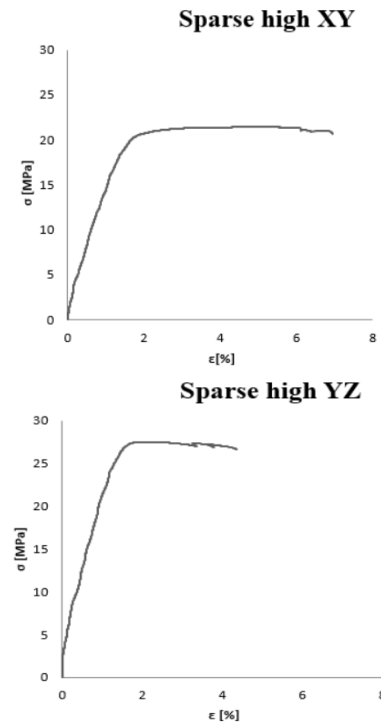
Figure 8. Average tensile strength - sparse high XY YZ.
