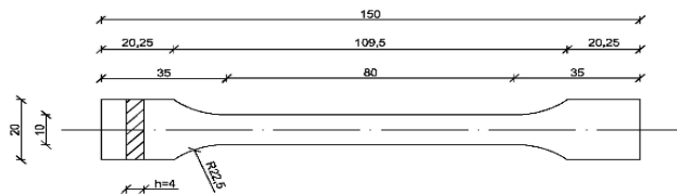
Figure 2. Paddle-shape sample dimensions.
