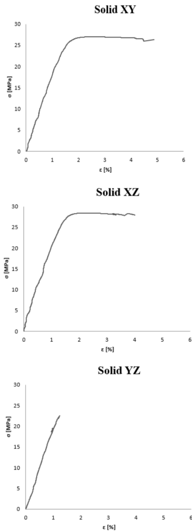
Figure 7. Average stress strain curve - solid XY, XZ and YZ.
