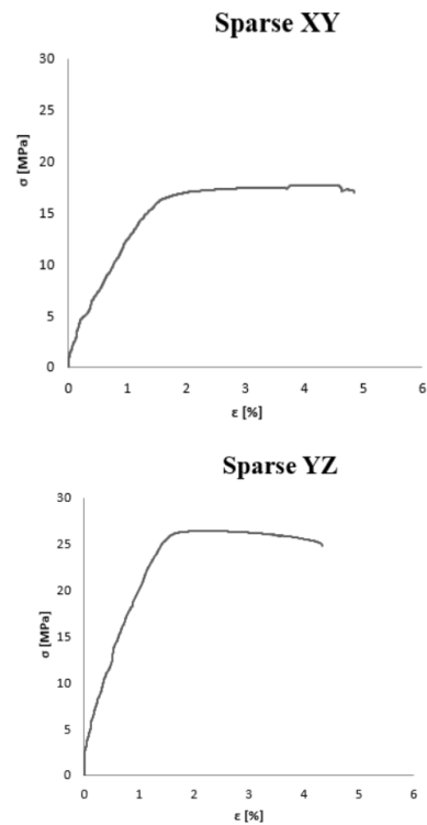
Figure 9. Average tensile strength - sparse XY and YZ.
