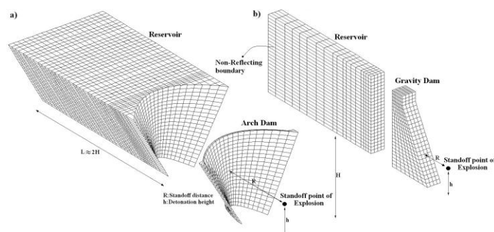
Figure 1. Concrete dam-reservoir finite element model subjected to air blast loading a) Arch dam –reservoir b) Gravity dam- reservoir
