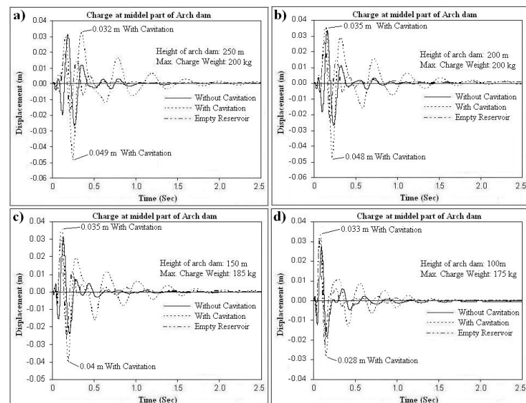
Figure 9. Crest displacement time histories at the point A for different dam heights subjected to air blast located at the middle part of downstream face of arch dam: a) H=250 m; b) H=200 m; c) H=150 m; d) H=100 m
