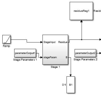
Fig. 5. Higher level of first pipeline stage.
