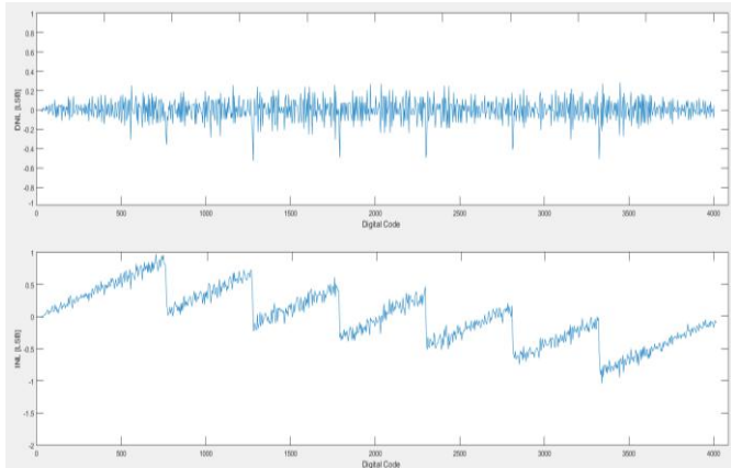
Fig. 14. DNL – INL plots without calibration.
