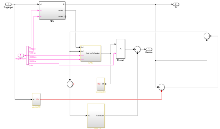
Fig. 8. Simulink conceptual foreground scheme on the exemplary stage.
