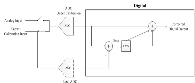
Fig. 2. Foreground calibration (LMS: Least Mean Square) [6].
