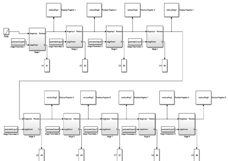
Fig. 4. Higher level design of pipeline ADC – 9 stages, 1.5 bits per stage.
