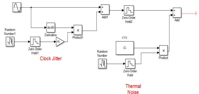
Fig. 12. Matlab implementation of clock jitter and thermal noise [10-11].
