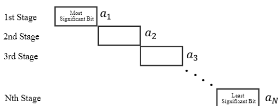
Fig. 3. An N-bit, ideal ADC with 1-bit per stage architecture.
