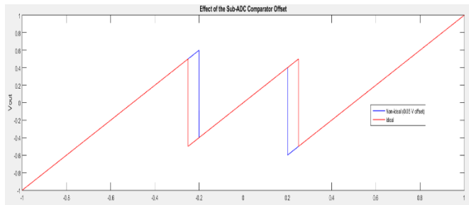
Fig. 9. The effect of the offset.
