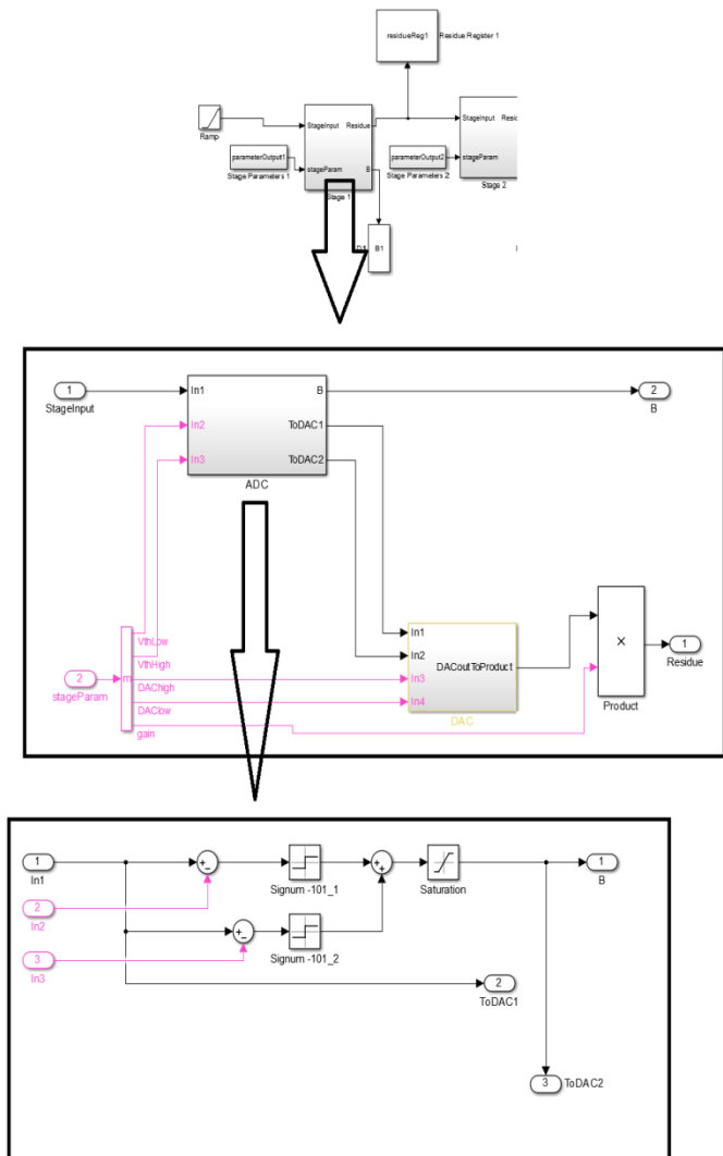
Fig. 6. Higher details of the each stage – ADC [8].
