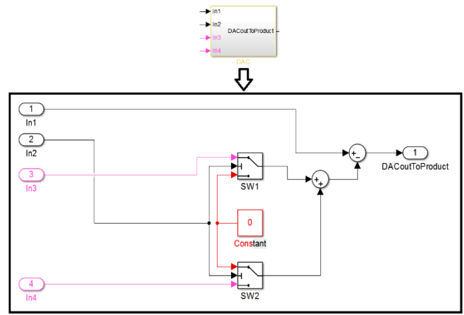
Fig. 7. Higher details of the each stage – DAC [8].
