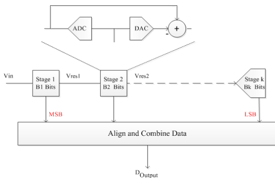
Fig. 1. Pipeline ADC Block Diagram.
