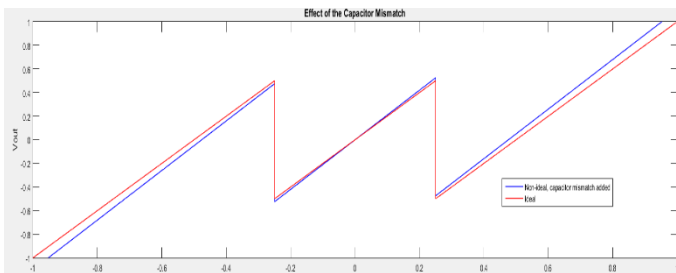
Fig. 10. The effect of the capacitor mismatch.
