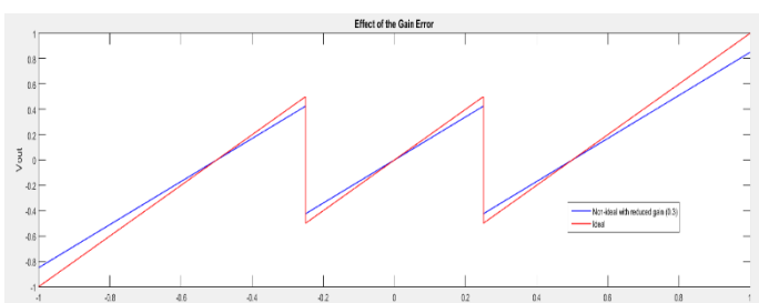
Fig. 11. Effect of the gain error accordingly the ideal case.
