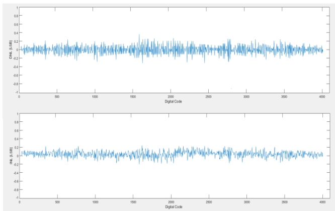
Fig. 15. DNL – INL plots with calibration.
