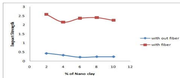
Fig. 11 Impact Strength vs. % of Nano Clay
