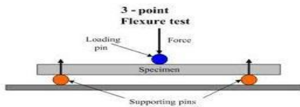
Fig. 5 Flexural testing arrangement
