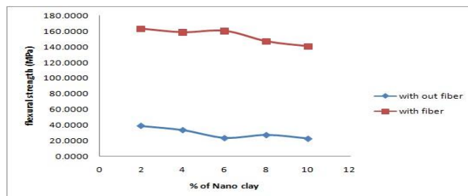
Fig. 10 Flexural Strength vs. % of Nano Clay
