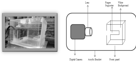
Fig.1 Finger Knuckle Capture Device
