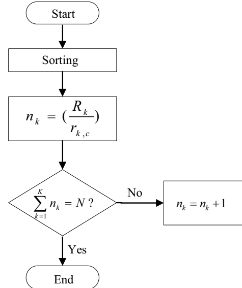
Figure 3: Flow chart for resource allocation to users.
