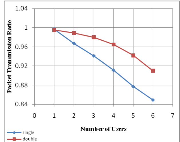
Figure 5. Packet transmission ratio vs. number of users for single and double line topologies
