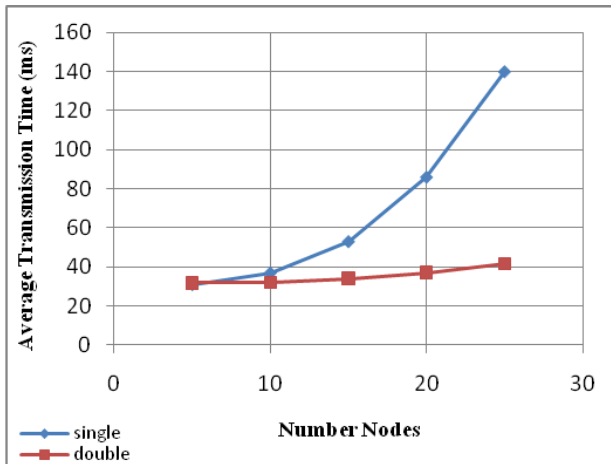
Figure 10. Packet transmission time delay vs. number of nodes for single and double line topologies
