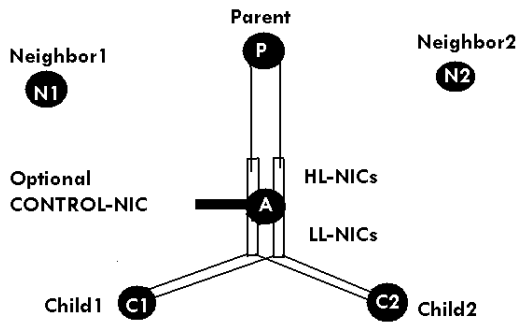
Fig. 6 Eliminate channel dependency by separating the set of NICs
