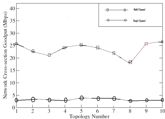
Fig. 7 Network Cross-Section Goodput is increase in Multi-Channel as compare in Single-Channel
