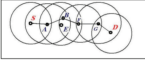
Figure 1. An established route in CR-MANETs
