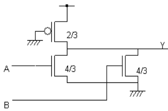
Figure 2. Pseudo-NMOS NOR gate
