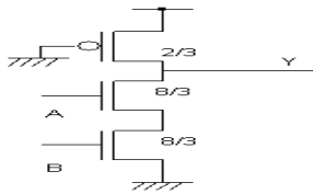
Figure 1. Pseudo-NMOS NAND gate
