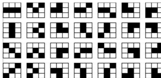
Fig. 3: Comparisons of central pixel to its two neighbor's pixels in 3 \times 3 Window
