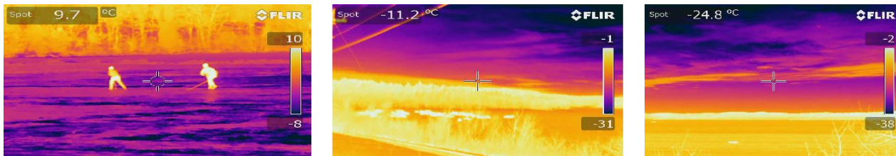
FIG. 1: infrared ice images with varying temperature range.
