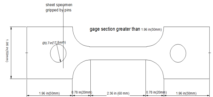
Figure 2. The geometric configuration of used sheet sample in this study, according to ASTM E8M standardization.
