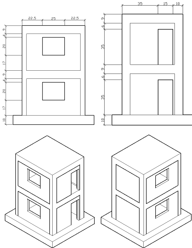
Fig 3. Dimensional of the Specimen 2(window opening)
