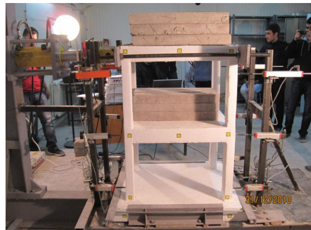
Fig 1. General photo of the test setup for the experimental study.
