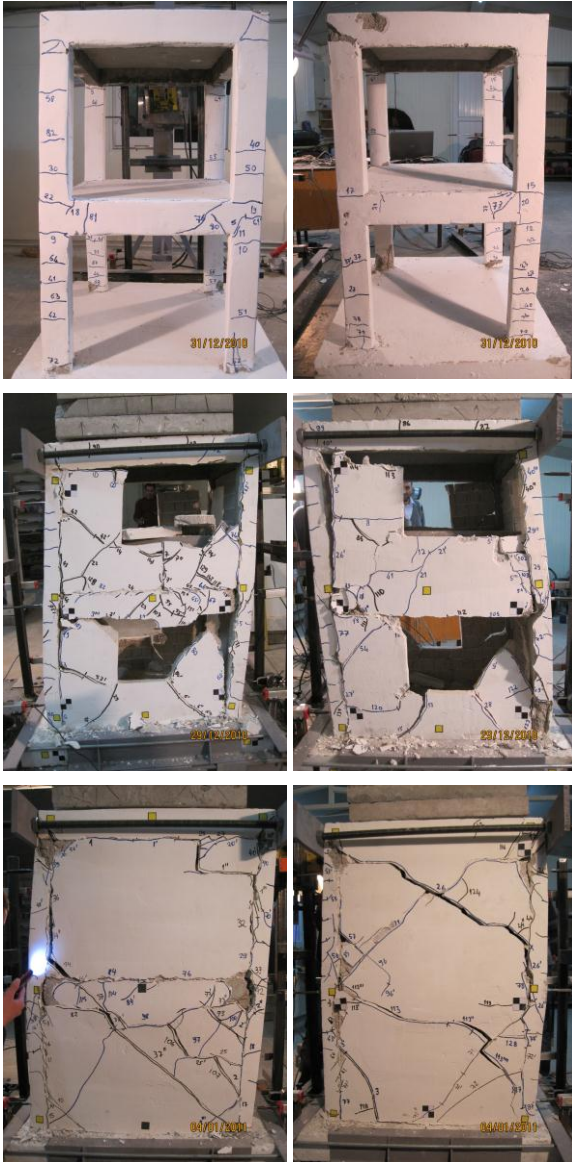
Fig 5. Specimen 1 (reference specimen), Specimen 2 (window opening) and Specimen 3 (no window opening) can be seen at the end of the test, respectively.
