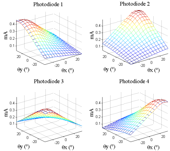
Figure 15. Generated photocurrents in sensor C.
