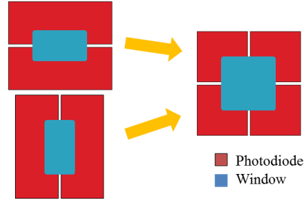
Figure 5. New 4-Quadrant structure.
