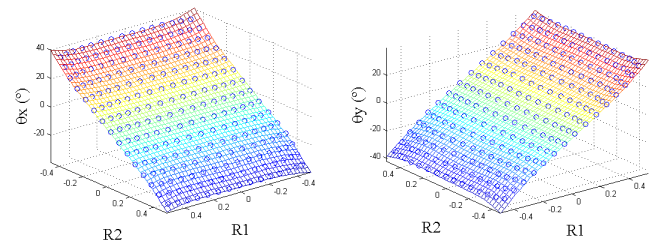
Figure 17. Inverse functions in sensor C.
