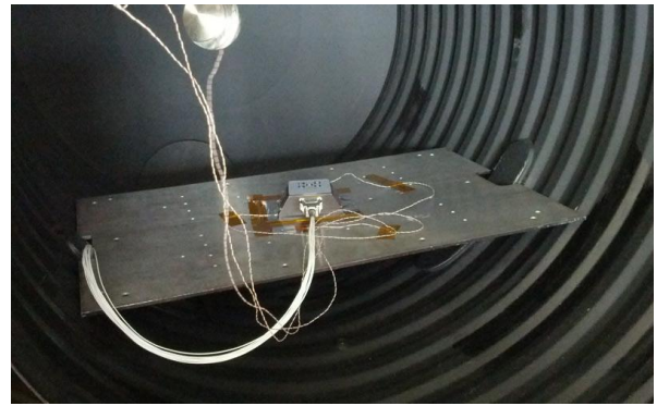
Figure 14. Climatic chamber thermal vacuum test.
