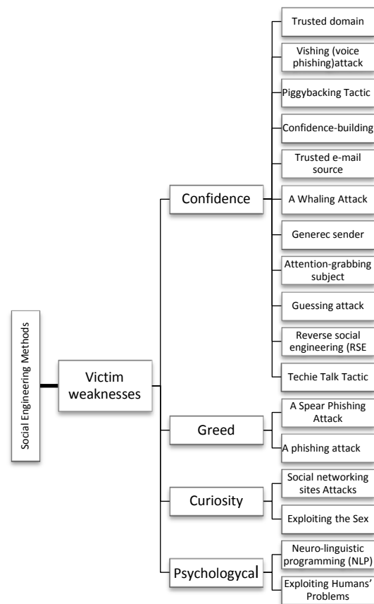
Figure 1. SEM classification.
