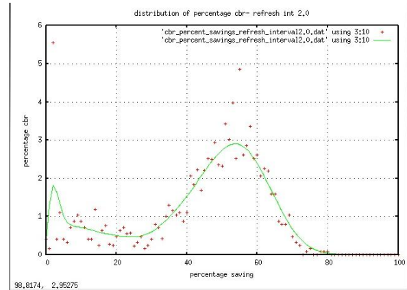
Fig 7: Distr. of %cbr for energy saving, RI 2.0 sec
