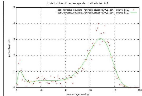
Fig 1: Distr. of %cbr for energy saving, RI 0.1 sec
