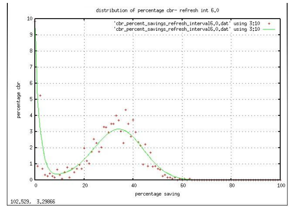
Fig 15: Distr. of %cbr for energy saving, RI 6.0 sec
