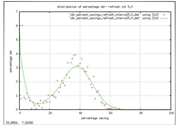
Fig 13: Distr. of %cbr for energy saving, RI 5.0 sec
