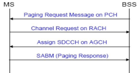
Figure 1: Paging Procedure
