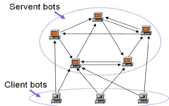
Figure 1: clustering
