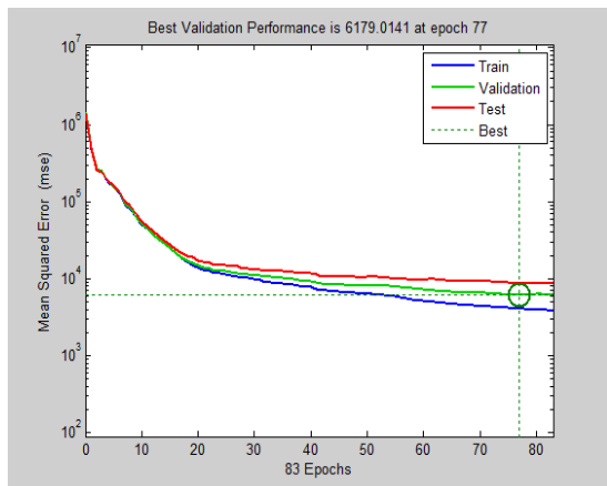
Figure 3. Performance Plot after training, validation and test.
