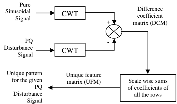
Figure 2. Algorithm for generating signatures of PQ disturbances
