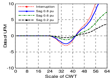
Figure 5. Patterns for interruption and sag - 0.2, 0.6 and 0.8 pu.
