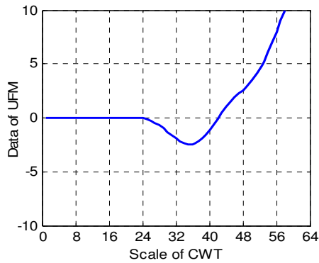
Figure 6. Signature for interruption and sag
