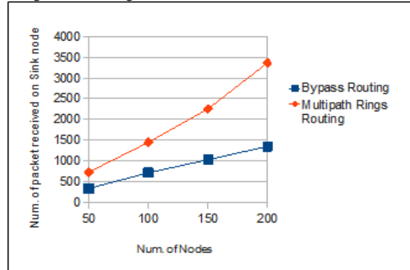
Figure 7. Comparison between Multipath rings routing and Bypass routing.
