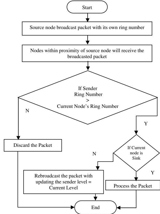
Figure 5. Execution of data dissemination phase in Multipath rings routing protocol.
