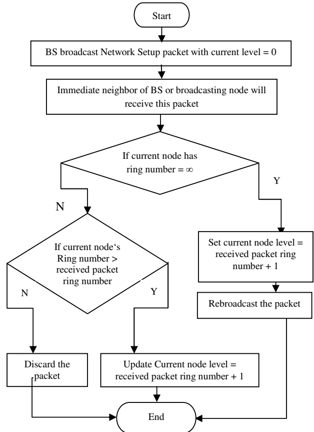
Figure 3. Flow chart of Topology setup phase
