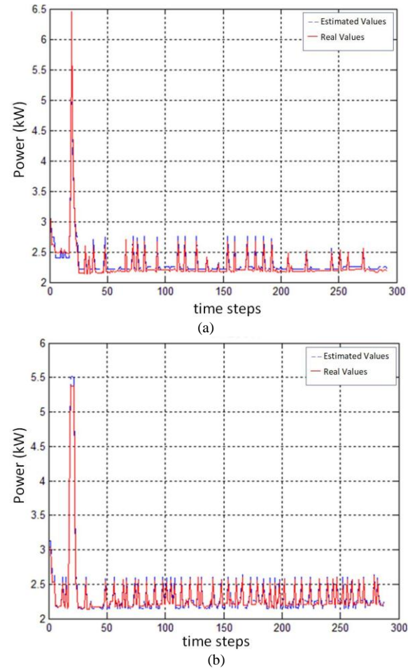
Fig. 3. Comparison of AHU power consumptions between estimated and real values for (a) AHU 1, (b) AHU 2.
