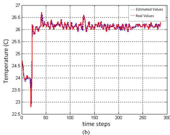
Fig. 3. Comparison of predicted and real AHU outlet cold air temperature for (a)AHU 1, (b) AHU 2.
