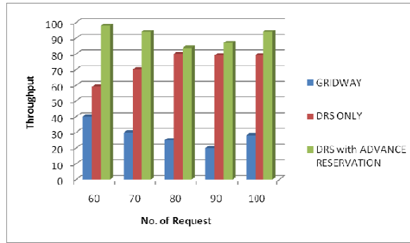
Figure 3. Number of request VS Throughput.
