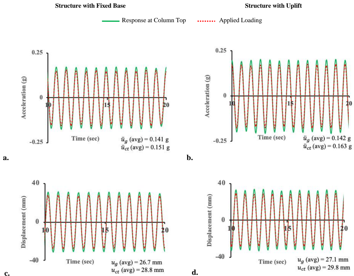
Figure 3. Column response for intermediate 10 seconds a. Acceleration-time history of SWFB, b. acceleration-time history of SWU, c. displacement-time history of SWFB, and d. displacement-time history of SWU
