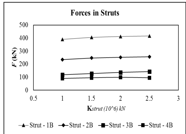
Figure 7: Forces in Strut for arrangement B
