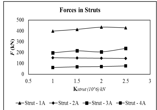
Figure 6: Forces in Strut for arrangement A
