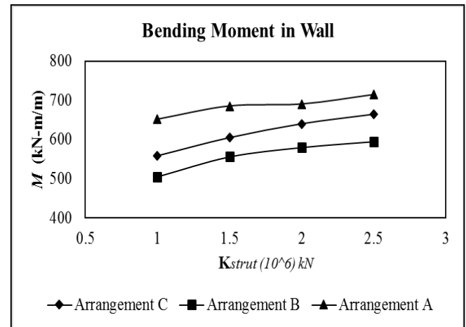
Figure 5: Variation in Bending moment in diaphragm wall with varying K_{strut}
