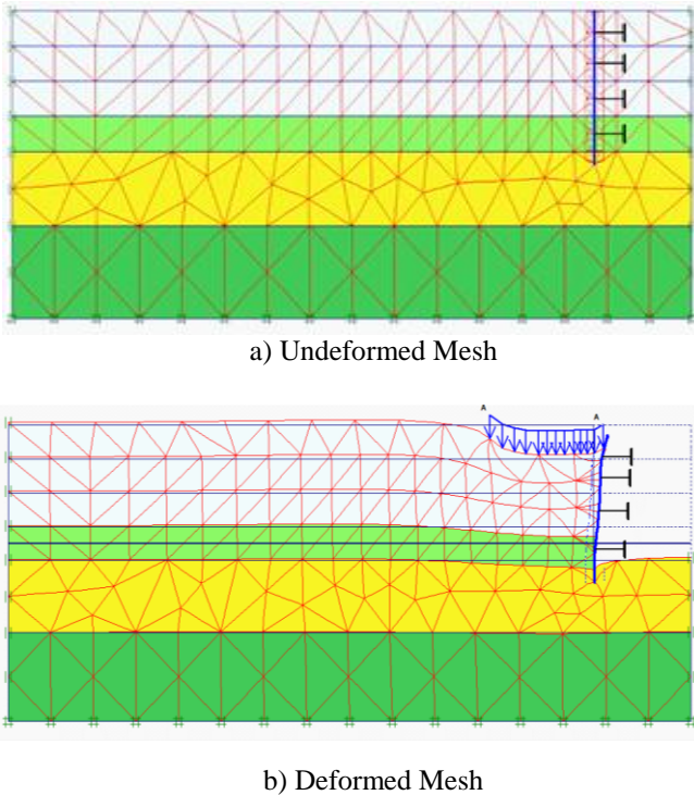
Figure 1: Mesh generation of diaphragm wall supported with horizontal struts
