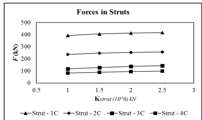
Figure 8: Forces in Strut for arrangement C
