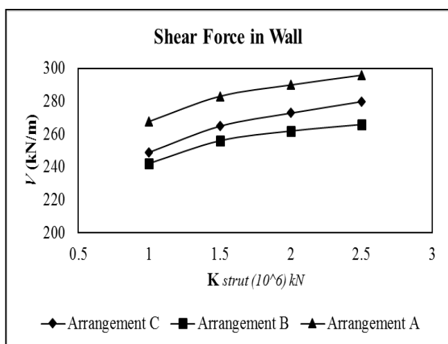
Figure 4: Variation in Shear force in diaphragm wall with varying K_{strut}
