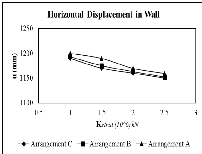
Figure 3: Effect of K_{strut} on horizontal displacement of diaphragm wall
