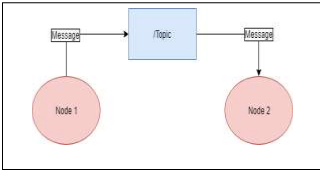
Figure 2. ROS architecture 1
