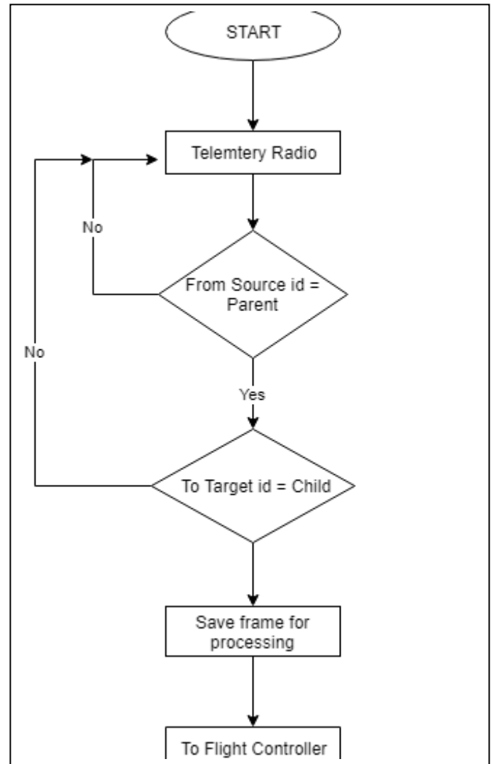
Figure 3. Relay communication approach for Child node
