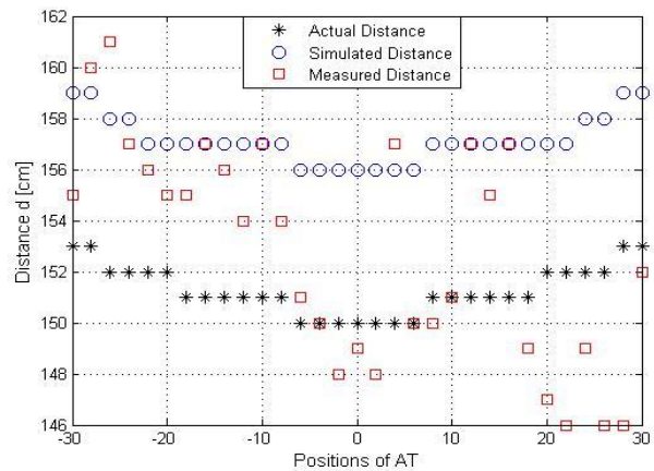
Figure 6. Radial distance d
