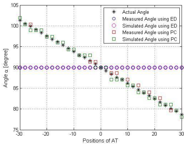
Figure 8. Azimuth angle \alpha
