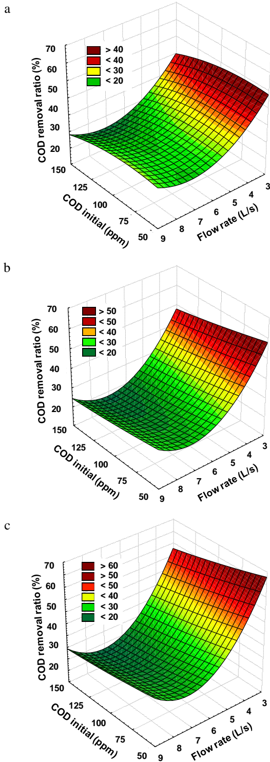
Figure 3: Effect of using a) gravel, b) star-shaped, and c) pall rings biofilters on the stream COD removal efficiency. The highest COD removal ratio occurred at the lowest flow rate (3 L/s). Moreover, the pall rings recorded the highest removal ratio, where the star-shaped came on the second place surpassing the values obtained by the gravel biofilters.
