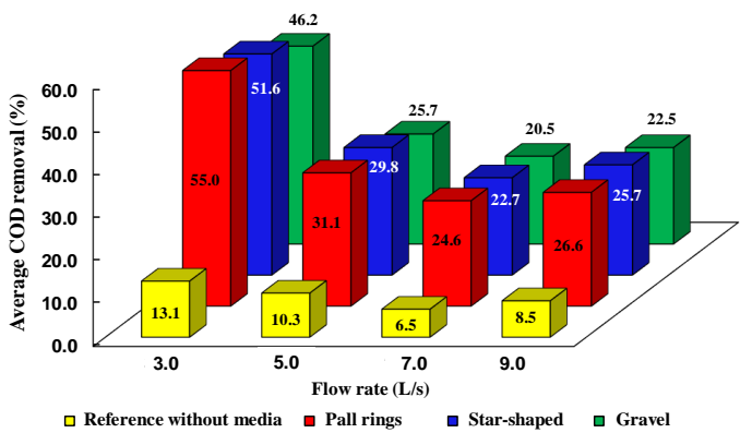
Figure 4: Effects of using different medias compared to the reference stream on COD removal ratio at different flowrates. On the meanwhile, the reference natural self-purification (without media) stream showed the lowest COD removal ratios. Thus, using the pall rings biofilters increased the efficiency of COD removal from 26.6 to 55.0% compared to 6.5 to 13.1% achieved by the natural self-purification in the reference channel.
