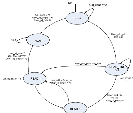
Figure 6: FSM for user read interface
