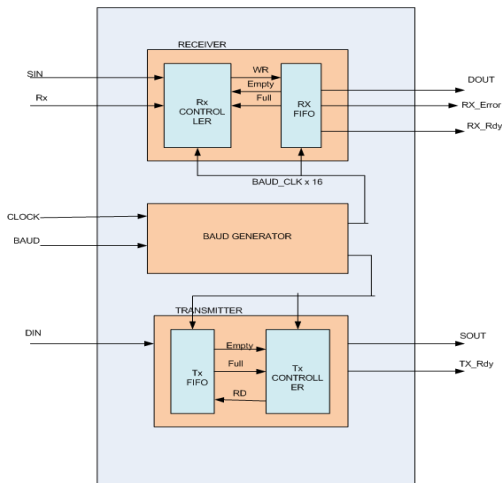
Fig. 2 Block diagram of UART
