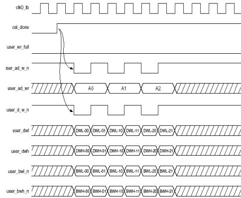
Figure 3: User write interface, ref [4]
