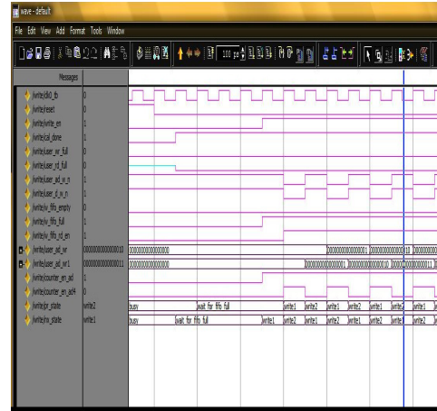
Figure 7: QDRII User Write Simulation result
