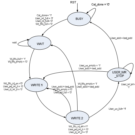
Figure 5: FSM for user write interface
