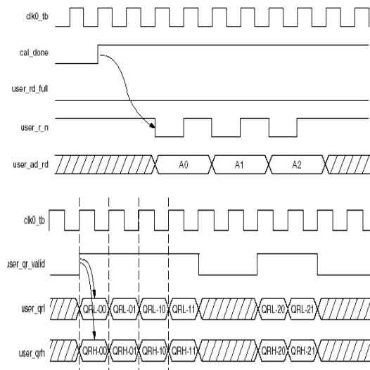
Figure 4: User Read interface, ref [4]
