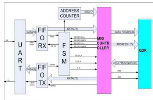
Fig. 1 Block Diagram of QDR II SRAM Interface
