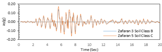
Figure 21. a_y(g) at center of footing for soil classes (Loma Prieta, 1989)
