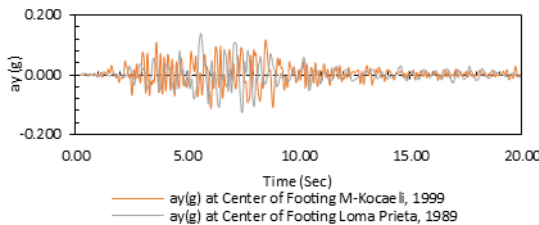
Figure 12. Seismic response a_y(g) at center of footing (Soil Class B)
