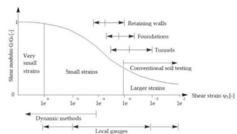
Figure 6. Characteristics stiffness-strain behavior of soil with typical strain ranges for laboratory [40]
