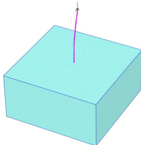
Figure 8. Vistas V47/660 at Zafarana 3 (Soil Class B) in Plaxis 3D
