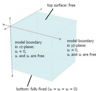
Figure 1. Default Boundaries in Plaxis 3D
