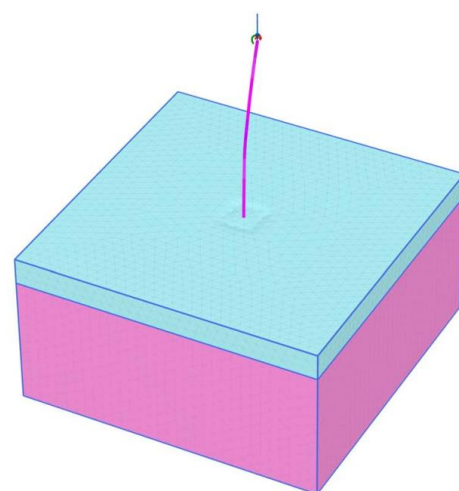
Figure 9. Vistas V47/660 at Zafarana 5 (Soil Class C) in Plaxis 3D
