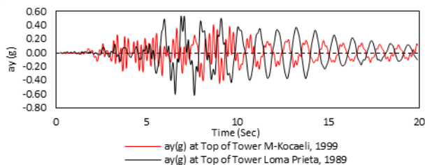
Figure 13. Response a_y(g) at top of tower (Soil Class B)
