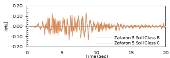
Figure 18. a_y(g) at center of footing for soil classes (Kocaeli, 1999)
