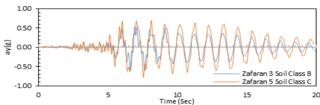
Figure 22. a_y(g) at top of tower for soil classes (Loma Prieta, 1989)
