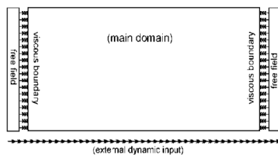
Figure 5. Free field boundary condition with rigid base (wave reflection at base) [38]
