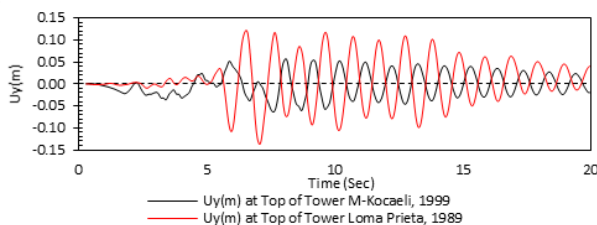
Figure 14. Response U_y(m) at top of tower (Soil Class B)
