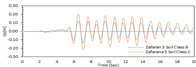
Figure 23. U_y(m) at top of tower for soil classes (Loma Prieta, 1989)
