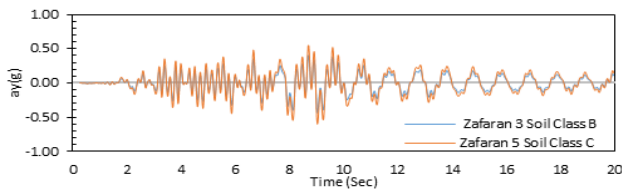
Figure 19. a_y(g) at top of tower for soil classes (Kocaeli, 1999)
