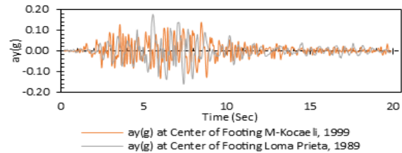
Figure 15. Seismic response a_y(g) at center of footing (Soil Class C)
