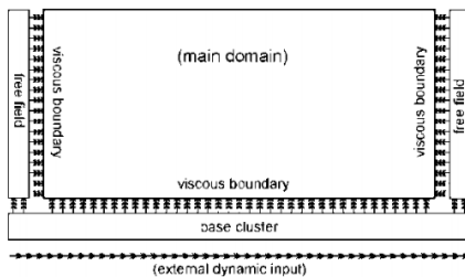
Figure 4. Free field boundary condition with compliant base (no wave reflection at base) [38]
