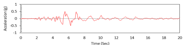
Figure 11. The Loma Prieta, 1989 scaled record to 0.50g PGA
