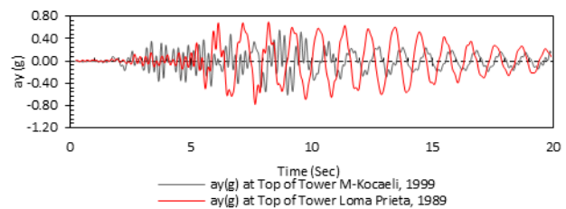
Figure 16. Response a_y(g) at top of tower (Soil Class C)
