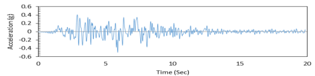
Figure 10. The Kocaeli, 1999 scaled record to 0.50g PGA
