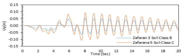
Figure 20. U_y(m) at top of tower for soil classes (Kocaeli, 1999)
