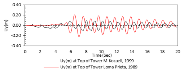
Figure 17. Response U_y(m) at top of tower (Soil Class C)
