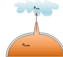
Fig. 5 Mass flow through Bleeder
