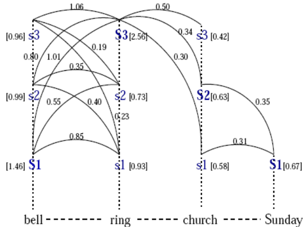
Figure 2. The label graph for assigning senses to words in the sentence used as an example. (from [6])
