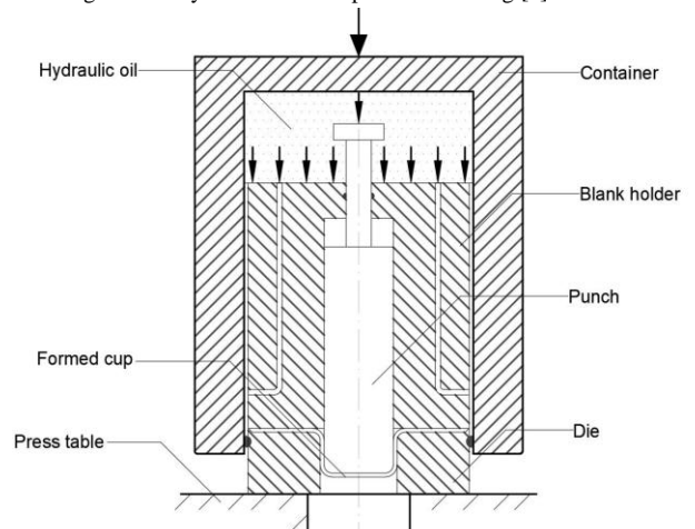
Figure 3. Hydraulic pressure-augmented drawing [11]
