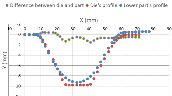
Figure 11. Comparison between the part and die profile, 10.5 mm die depth
