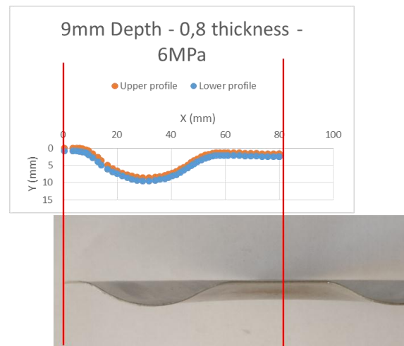
Figure 8. Upper and lower profile of the part
