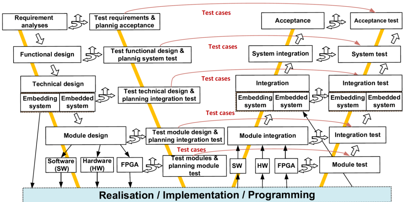
Figure 4: W-Process Model (from [7])
