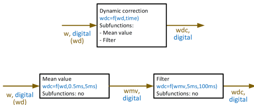
Figure 7: Design Example Dynamic Correction, Middle and Lower Level
