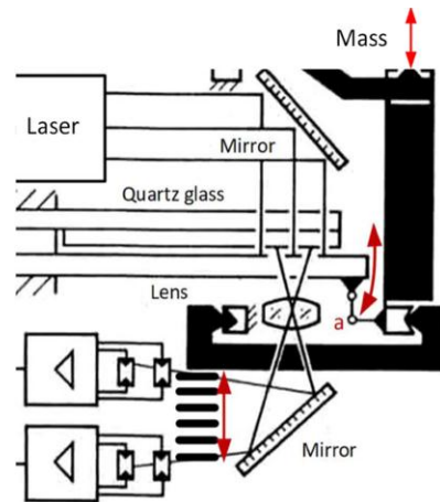
Figure 1: Weighing Machine: Prototype Schematic (partly from [2])
