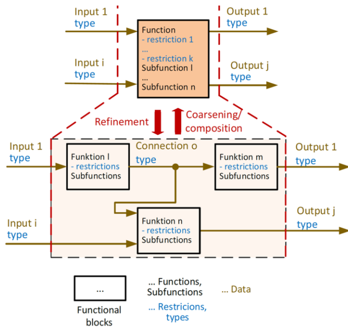
Figure 5: Function Blocks and Various Abstraction Levels
