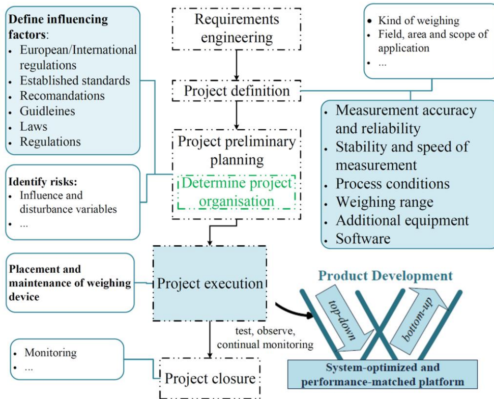
Figure 9: Project Management and W Process (from [7])
