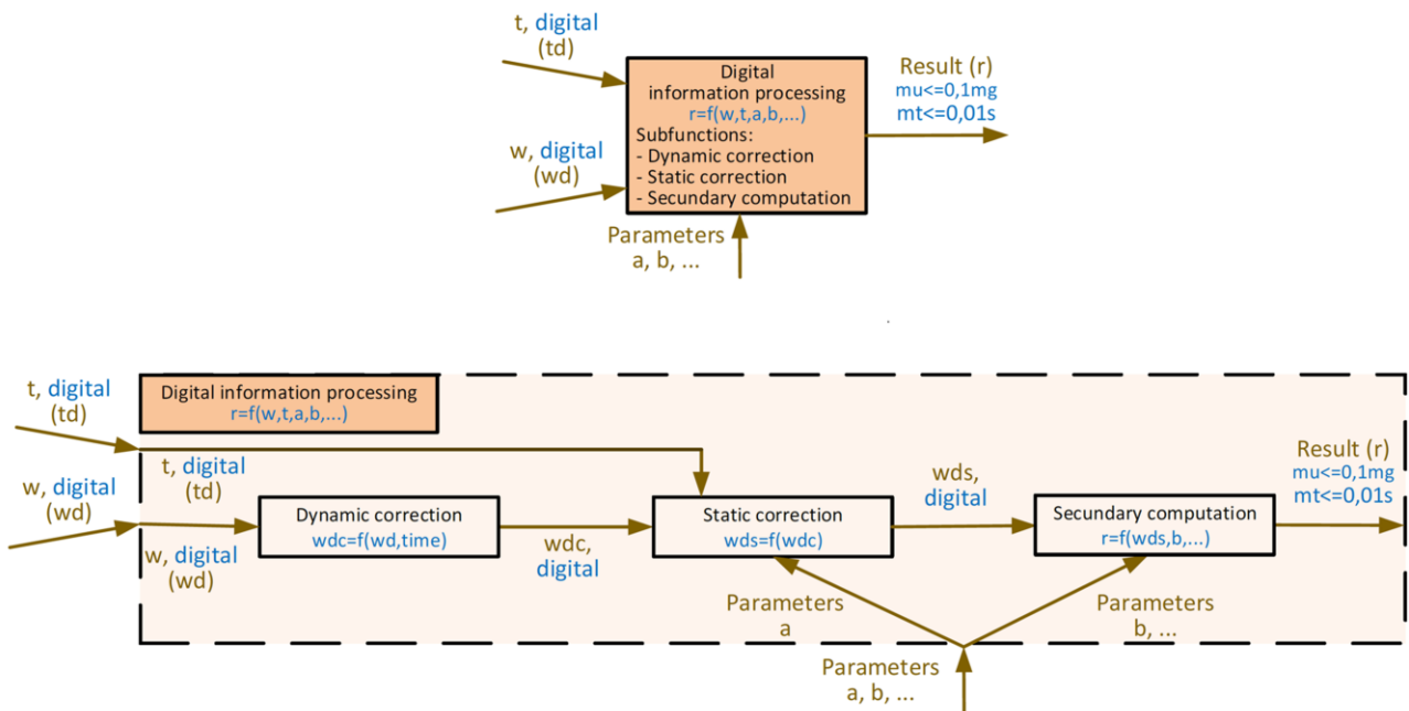
Figure 6: Design Example Digital Information Processing, Higher and Middle Level
