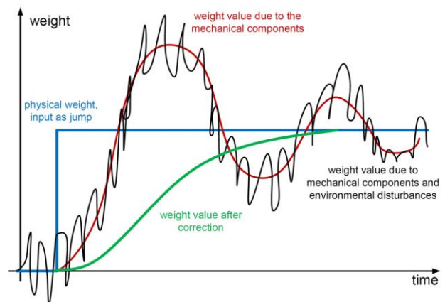
Figure 3: Weight Value After Several Corrections
